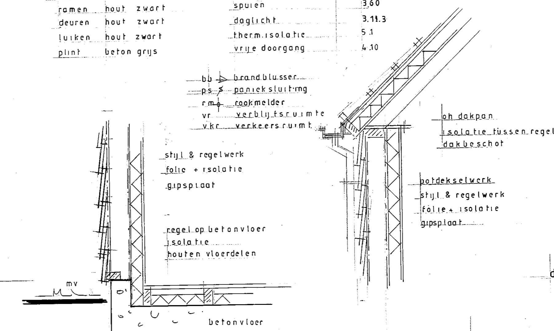
details 1:20
